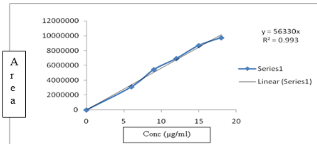
Fig 6: Graph of linearity
