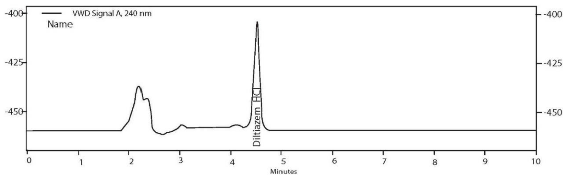
Fig 5: Specificity Sample chromatogram of Diltiazem HCl
