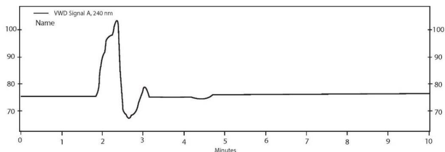
Fig 2: Chromatogram for diluent
