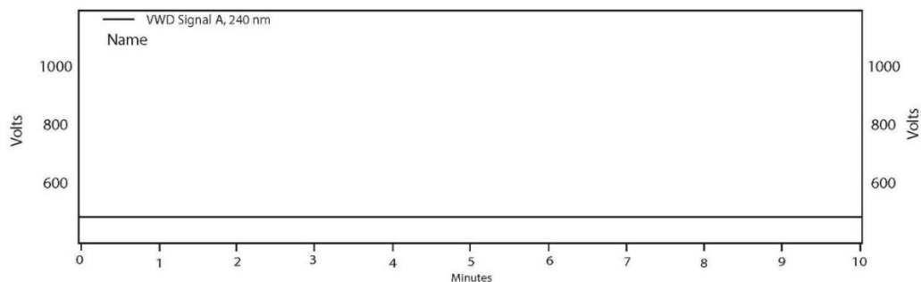
Fig 3: Chromatogram for blank
