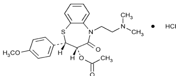
Fig 1: Structure of Diltiazem HCl
