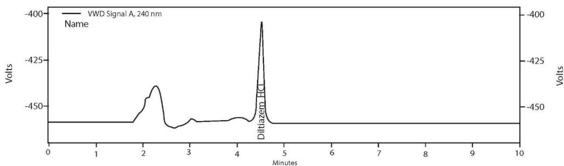
Fig 4: Specificity Standard chromatogram of Diltiazem HCl
