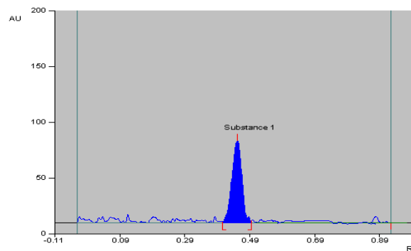
Fig. 1: Typical densitogram of Linagliptin (Rf 0.48 ± 0.5)
