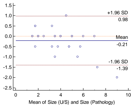
Fig. 2: Bland and Altman plot, showing the agreement between tumour size measured by ultrasound and by pathologic examinations
