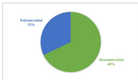
Fig. 1: Isolates
