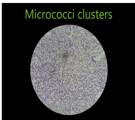
Fig. 10: Micrococci clusters
